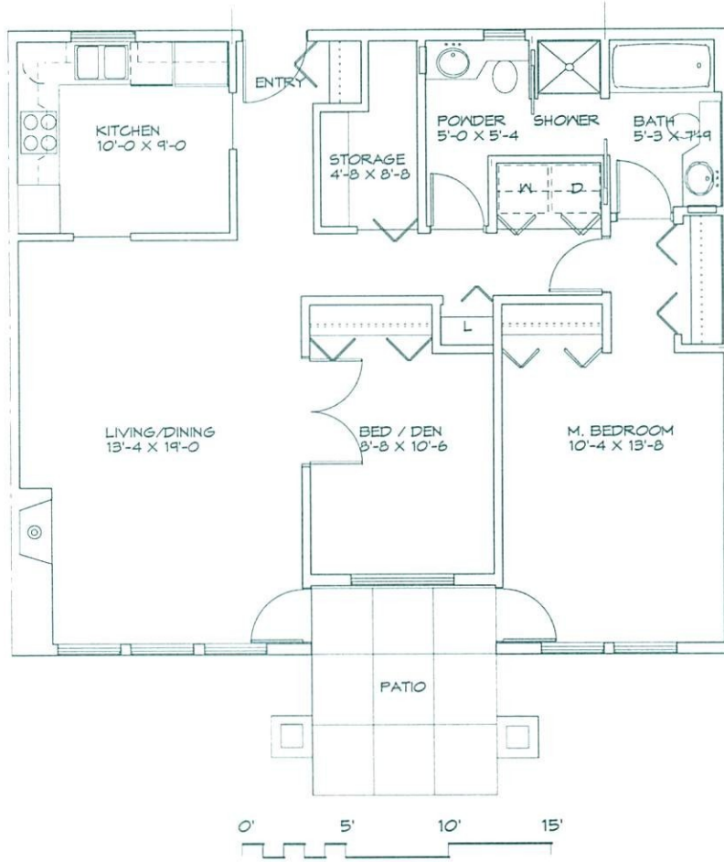
UNIT TYPE 'B' • LEVEL ONE FLOOR AREA - 978.5 SQ.FT.
